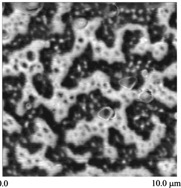
FIG. 1. MFM image of a multilayer CoPt on YBCO, showing maze-like domain structure with uniaxial perpendicular magnetic anisotropy.
