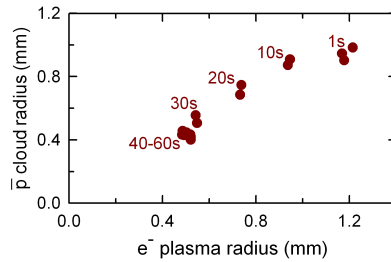
FIGURE 5. The \bar{p} cloud radius as a function of the e^- plasma radius for the slow compression data shown in Fig. 4.
