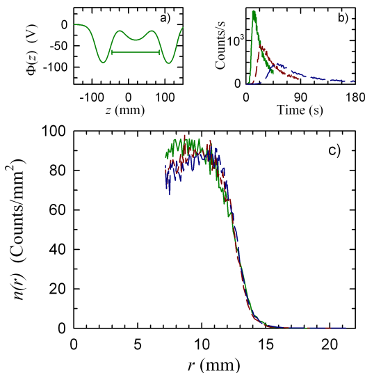
FIGURE 9. Comparison of the radial profiles with octupole ramps of 45 (green solid), 90 (red short-dash), and 180 s (blue long-dash). Panel a) shows the electrostatic well potential \Phi(z) ; the horizontal bars indicate the 130 \pm 5 mm axial extent and position of the \bar{p} orbits before the application of the octupole field. Panel b) shows the time history of the \bar{p} annihilations as the octupole field is ramped up. Panel c) shows the resulting radial profiles. The maximum B_w , at the end of the ramp was 1.54 T, and B_z = 1.03 T.
