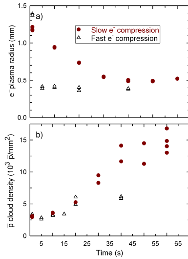
FIGURE 4. The a) e^- radius and b) \bar{p} density as a function of time, for fast and slow compression. Note that the \bar{p} density does not track the e^- compression if the latter is fast.
