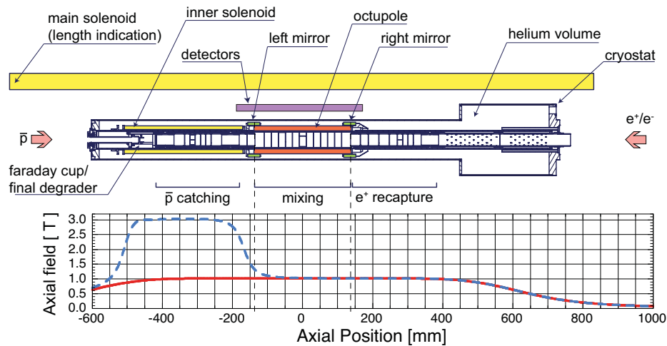
FIGURE 1. Schematic diagram of the ALPHA apparatus. A moveable probe on the right alternately inserts an electron gun and a MCP/Phosphor assembly. The graph below the schematic plots the axial magnetic field in the trap; the dashed line includes the field of the inner solenoid, while the solid line is the field without the inner solenoid.
