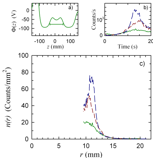
FIGURE 10. Comparison of the \bar{p} radial profile with different density positron plasmas. The green, solid curve shows the profile with no e^+ , and the red short-dash and blue long-dash curves show the profile with 13 million and 25 million e^+ respectively. The well length was 85 \pm 5 mm, the maximum field was 1.20T, and the ramp time was 20s. The graph descriptions and all other parameters are the same as in Fig. 9.
