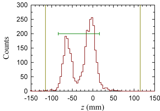
FIGURE 8. Axial positions where the \bar{p} 's hit the trap wall under the influence of the octupole. The horizontal bar indicates the the axial extent and position of the electrostatic well confining the \bar{p} 's. The loss is greatest near the ends of the confining electrostatic well. The positions are determined by a position-sensitive particle detector which monitors the \bar{p} annihilation products; the vertical bars indicate the axial extent of the detector.
