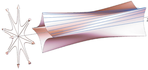
FIGURE 6. Magnetic field generated by the octupole and solenoid coils. The vectors on the left represent the directions of the axially-invariant field from these coils. The surface is created by following the field lines from a radially centered circular locus of points; the lines shown within the surface are field lines.
