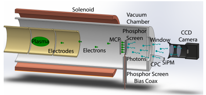
FIG. 1. Simplified schematic (not to scale) of the experiment. Electrons released from the plasma flow onto the MCP. Each plasma electron produces a cascade of up to 18 000 electrons in the MCP. These electrons are accelerated onto a fast phosphor (P47) screen to produce blue photons. The plasma signal can be read via the light collected by the compound parabolic light concentrator (CPC) and detected by the SiPM, or by the charge on the phosphor screen (FC). The CCD camera is used to determine the plasma radial density profile.
