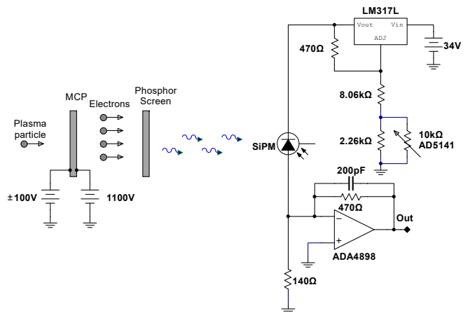
FIG. 5. Simplified schematic of the SiPM circuit.
