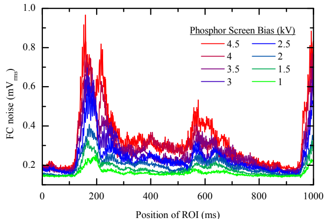
FIG. 4. FC noise due to microphonics related to the coldhead, and measured on the 1\text{ nF} capacitor in the circuit of Fig. 3 as a function of the phosphor screen bias. The RMS noise (minus DC offset) is measured for a 1\text{ ms} moving window (ROI), and averaged over 30 traces. Traces were collected with a trigger synchronized to the coldhead cycle.
