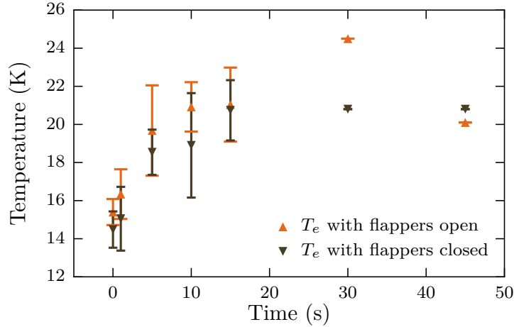
Figure 5.11: Electron temperature measurements made with the flappers open, indicated by the orange triangles (▲), and closed, indicated by the brown triangles (▼), in December 2017. The error bars show the standard deviation of five measurements.
