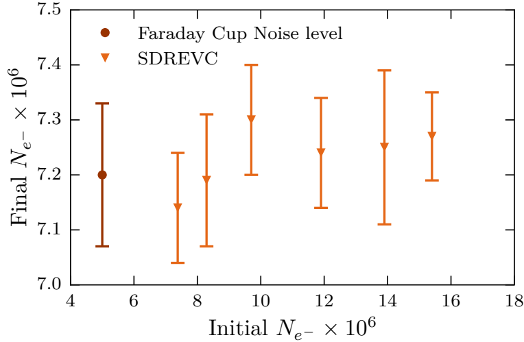
Figure 4.5: Magnified plot of the number of particles with SDREVC (▼) and the noise level of the Faraday cup detector (●).
