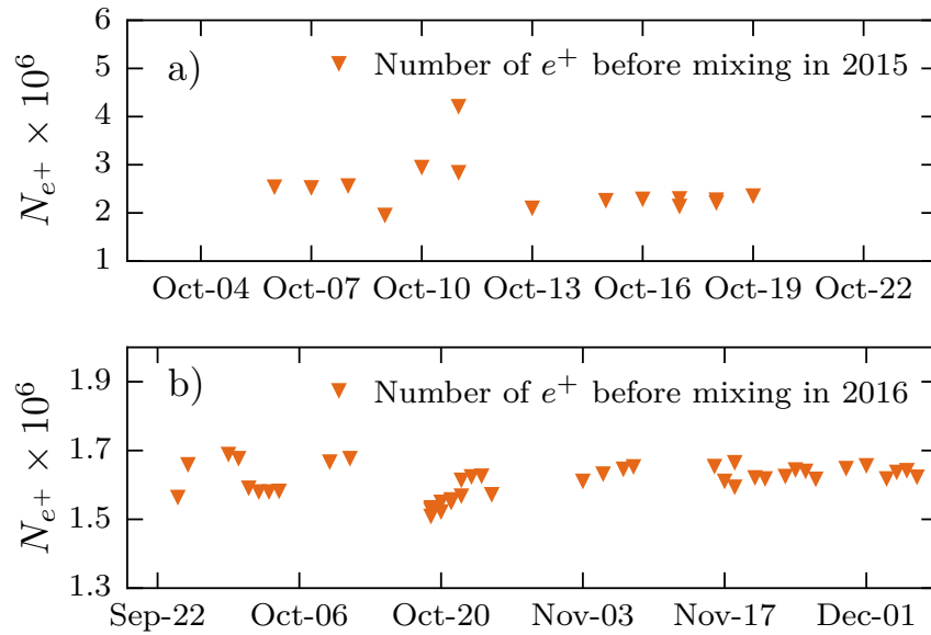
Figure 5.3: Measurements of the number of positrons just before mixing in (a) 2015 and (b) 2016, the same data as in Fig. ?? but magnified to show more detail.
