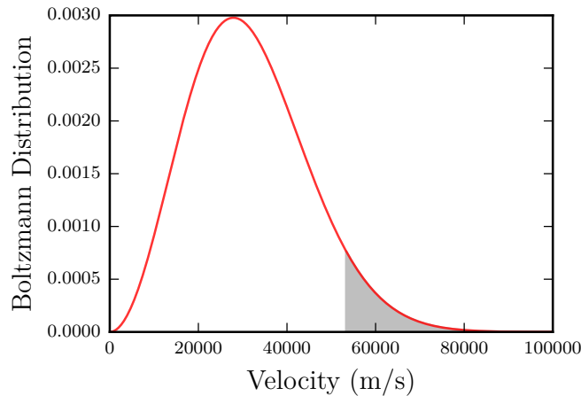
Figure 3.5: Normalized 3d Maxwell-Boltzmann distribution. The shaded region represents 6.3% of the particles that together constitute about 20% of the total energy.
