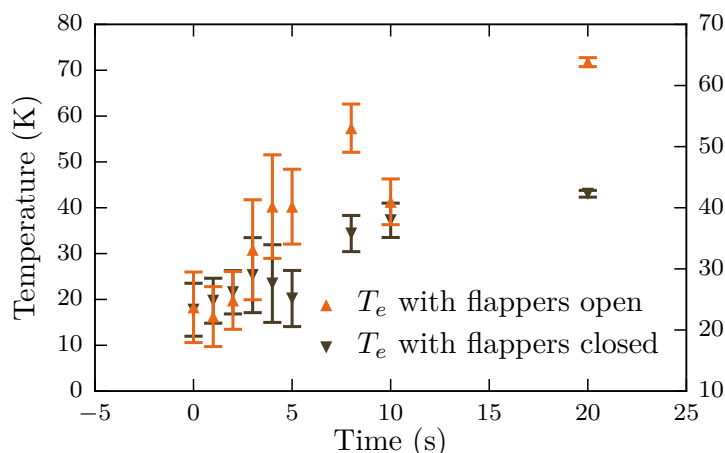
Figure 5.10: Electron temperature measurements made with the flappers open indicated by the orange triangles (▲) and closed indicated by the brown triangles (▼) in February 2017. The error bars show the standard deviation of 8 measurements.
