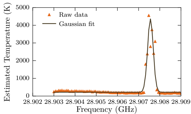
Figure 2.10: Plasma temperatures as a function of microwave frequency; the peak corresponds to the plasma ECR frequency and is used to directly determine the magnetic field.
