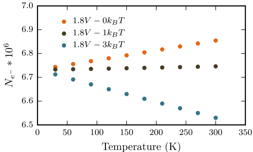
Figure 4.11: The calculated numbers of electrons, N_{e^-} , is plotted as a function of temperature. The curves correspond to different values of thermal energy k_B T .
