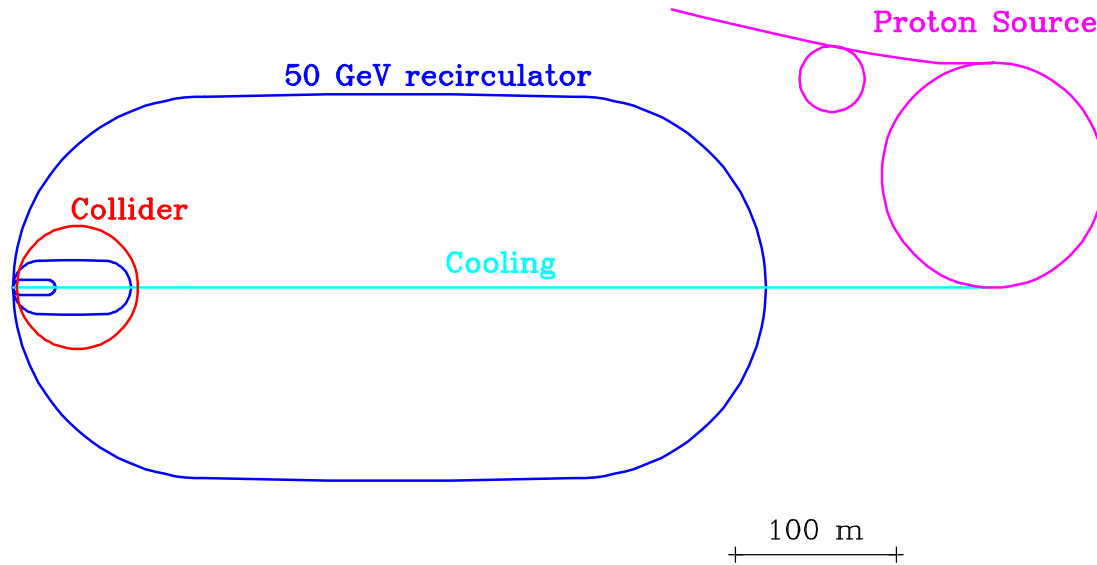
FIG. 28: Plan of a 0.1-TeV-CoM muon collider.
