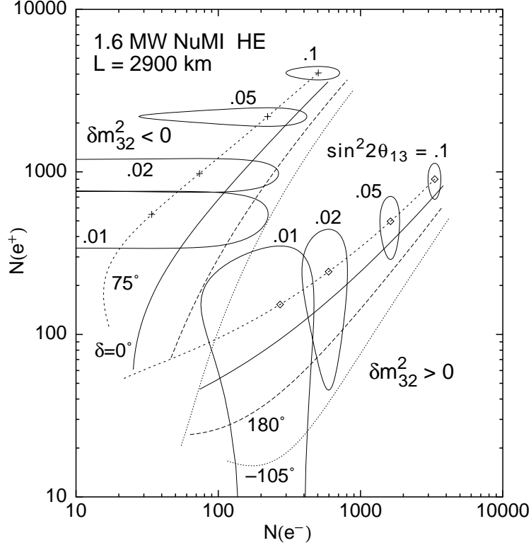
FIG. 7: Three-sigma error ellipses in the (N(e^+), N(e^-)) plane, shown for \nu_\mu \rightarrow \nu_e and \bar{\nu}_\mu \rightarrow \bar{\nu}_e oscillations in a NuMI-like high energy neutrino beam driven by a 1.6 MW proton driver. The calculation assumes a liquid argon detector with the parameters listed in [22], a baseline of 2900 km, and 3 years of running with neutrinos, 6 years running with antineutrinos. Curves are shown for different CP phases \delta (as labelled), and for both signs of \delta m_{32}^2 with |\delta m_{32}^2| = 0.0035 \text{ eV}^2 , and the sub-leading scale \delta m_{21}^2 = 10^{-4} \text{ eV}^2 . Note that \sin^2 2\theta_{13} varies along the curves from 0.001 to 0.1, as indicated [70].
