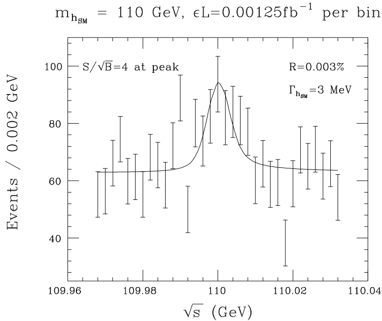
FIG. 10: Number of events and statistical errors in the b\bar{b} final state as a function of \sqrt{s} in the vicinity of m_{h_{\text{SM}}} = 110 \text{ GeV} , assuming R = 0.003\% , and \epsilon L = 0.00125 \text{ fb}^{-1} at each data point.
