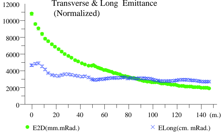
FIG. 17: The longitudinal and transverse emittances, obtained with the Geant4 [126] simulation code, as a function of channel length. The length of the lattice was extended by \approx 20 m to investigate the ultimate performance of the cooling channel.
