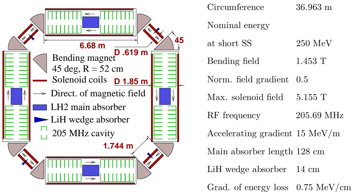
FIG. 29: Layout and parameters of the solenoid based ring cooler
