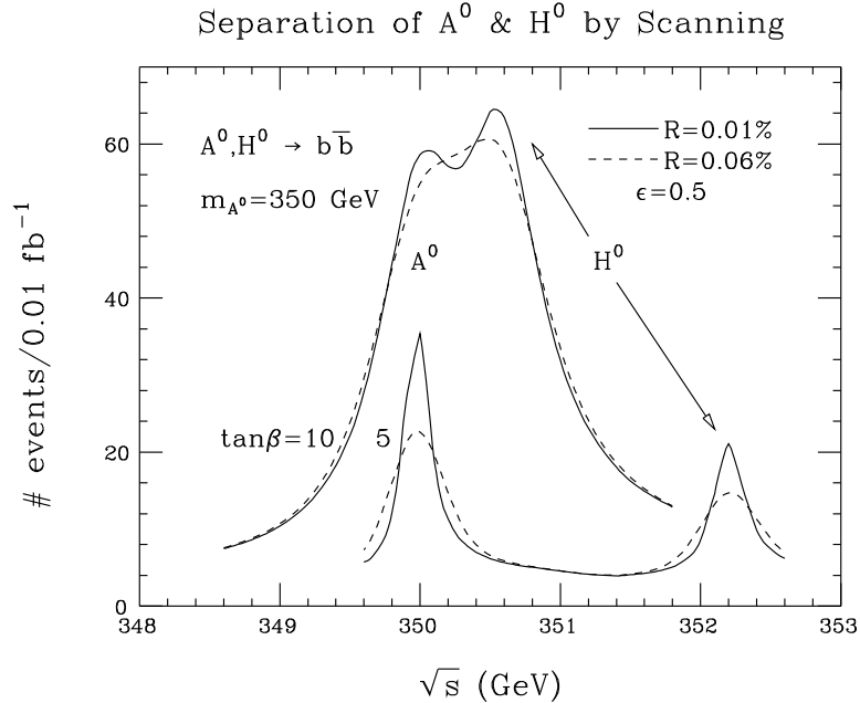
FIG. 11: Separation of A and H signals for \tan\beta = 5 and 10 . From Ref. [111].
