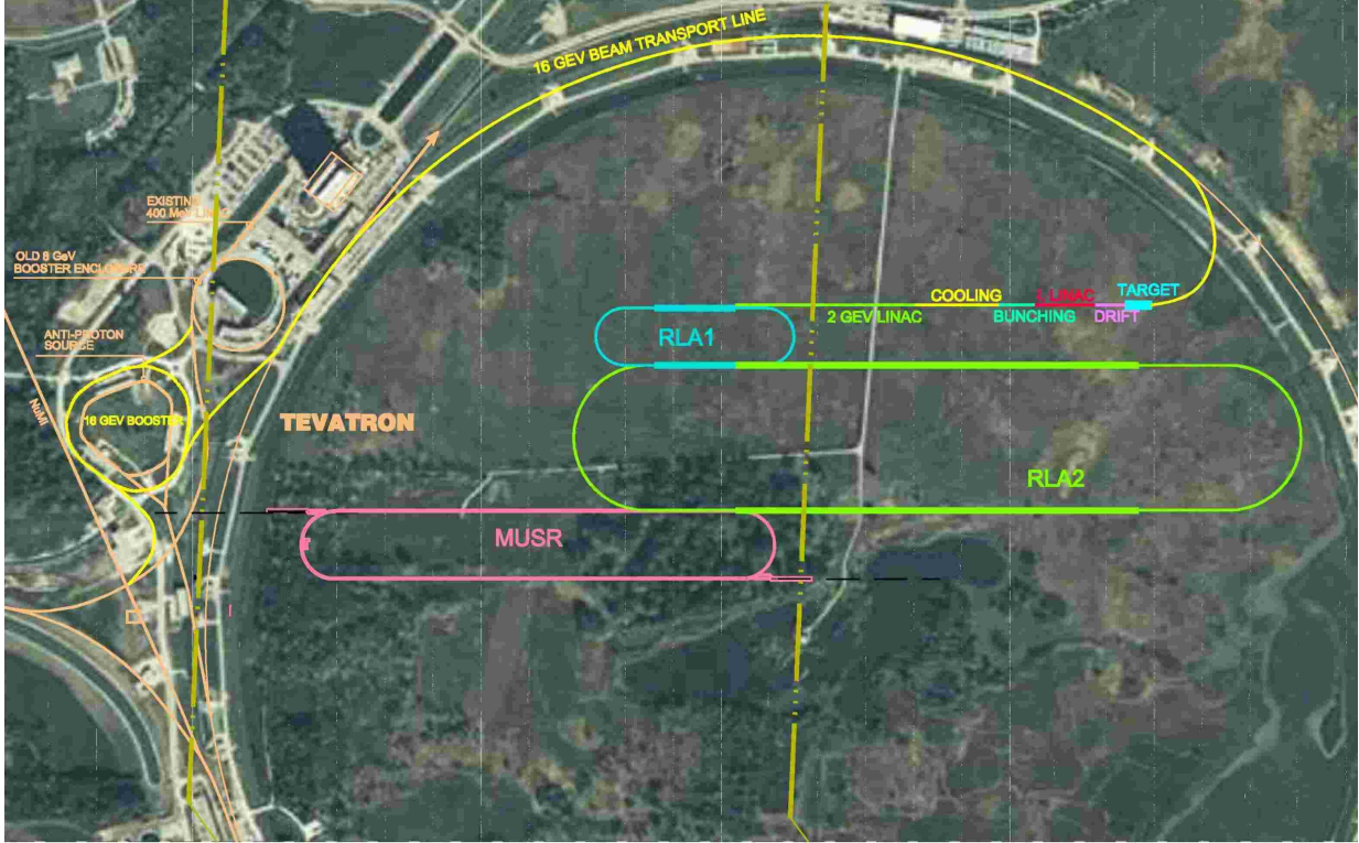
FIG. 23: Schematic of a 50-GeV Neutrino Factory at Fermilab.
