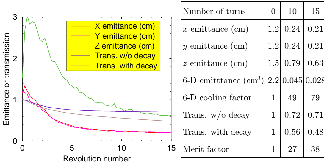
FIG. 30: Evolution of the beam emittance/transmission at the ring cooler.
