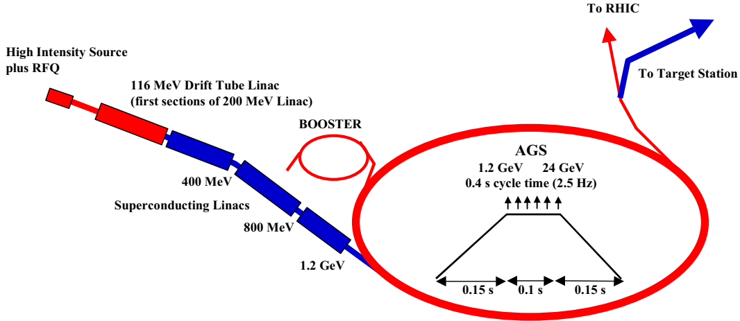
FIG. 12: AGS proton driver layout.
