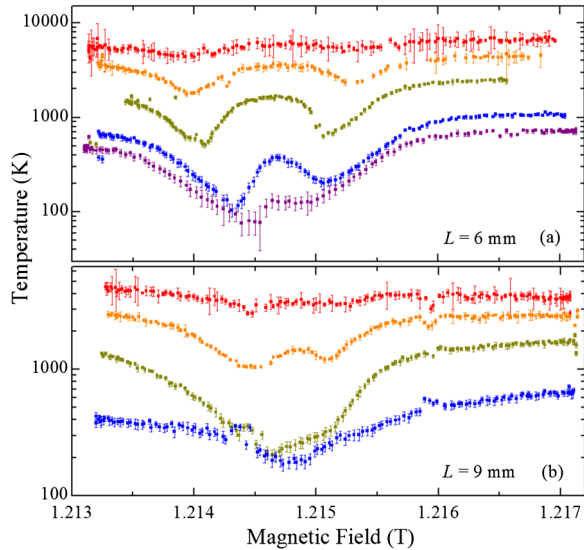
FIG. 4. Line shape splitting at TM_{031} as a function of plasma length L and temperature T . The confining potentials were set to produce 6 mm plasmas in (a) and 9 mm plasmas in (b). Plasma temperatures were measured after cooling for 0.1 s (red), 0.5 s (orange), 1.5 s (green), 4 s (blue), and 6 s (purple). The feature visible at 1.2159 T is from a reservoir reload.
