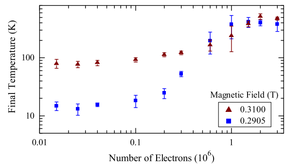
FIG. 5. Equilibrium temperature of plasmas with 10^4 – 10^6 electrons. In the dark red data set the field is detuned 19.5 mT (546 MHz) from the TE_{111} resonance.
