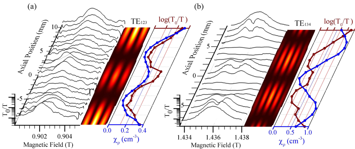
FIG. 3. Cooling enhancements: (a) TE 123 with 2 \times 10^4 electrons and (b) TE 134 with 3 \times 10^5 electrons. For each mode, the left waterfall plot shows the ratio T_0/T as a function of the magnetic field and plasma position ( T_0 is the typical off-resonant temperature for each data set). The central color contour plot shows the mode structure. The right-hand graph plots T_0/T at zero detuning [i.e., 0.902 T (a) and 1.436 T (b)] (red points), along with the overlap integral \chi_p defined by Eq. (3) (blue points).
