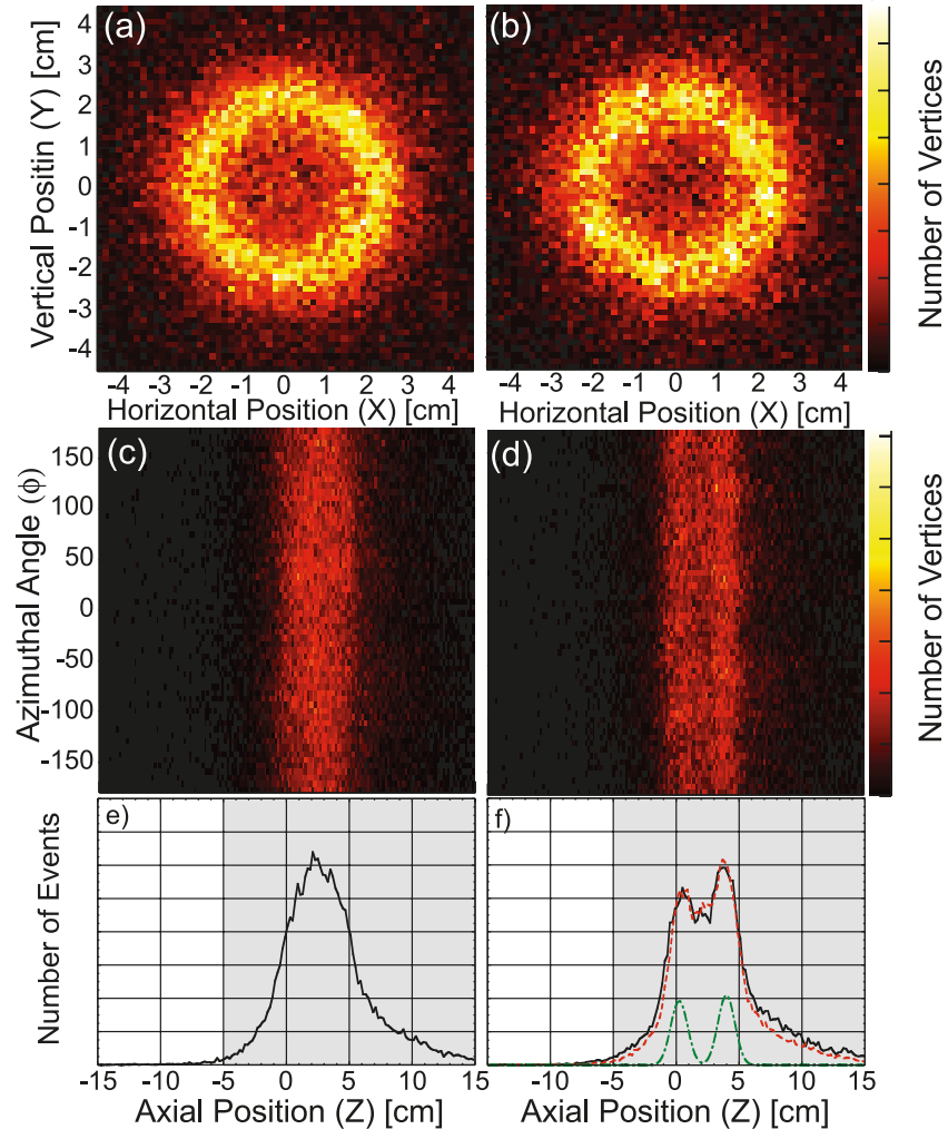
Fig. 2. Azimuthal projections of the antiproton annihilation vertex distributions during mixing with (a) no neutral atom trap and (b) the full trap. Corresponding z - \phi distributions. Corresponding axial ( z ) distributions. (f) Dashed (red): fit to the distribution, see text; dot-dashed (green) peaks in fit. The shaded area marks the three layer part of the detector used for tracking. Left of this area the detector has only one layer of silicon. The slight asymmetry in the axial distributions (in particular the tails) is due to the lower reconstruction efficiency outside the three layer section. For clarity the plots have been normalized to have the same total number of events. The total numbers of events with and without the neutral trap were 6830 and 26823, respectively. The zero axial position is the center of the neutral atom trap.
