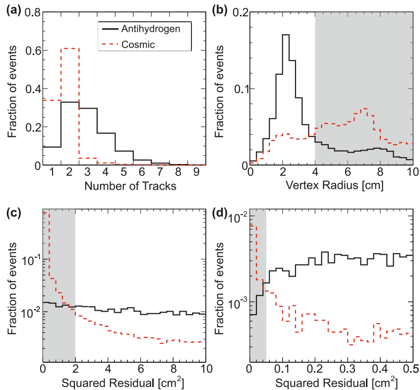
Fig. 7. Measured distributions of (a) the number of identified charged particle tracks, (b) the radial coordinate of the vertex, and the squared residual from a linear fit to the identified positions for the events with (c) two tracks and (d) more than two tracks. The distributions from antihydrogen annihilations are shown in solid black lines and from cosmic rays in dotted red lines. The shaded regions in (b), (c), and (d) indicate the range of parameters that are rejected.
