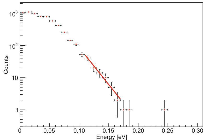
Fig. 4. Antiprotons lost as a function of trap depth. Annihilation events are counted while the trap depth is lowered over 100 ms. The detector has a 25\% \pm 5\% absolute efficiency for detecting an antiproton annihilation. The graph shows how many particles escaped at each point in this process. The temperature is extracted by fitting the release of the first approximately two hundred escaping particles, and the fit gave 219 \pm 33 K. The counting uncertainty is purely statistical, and the extracted temperature has not been corrected for adiabatic cooling nor space charge (see text). The horizontal uncertainty represents the energy resolution of the measurement.
