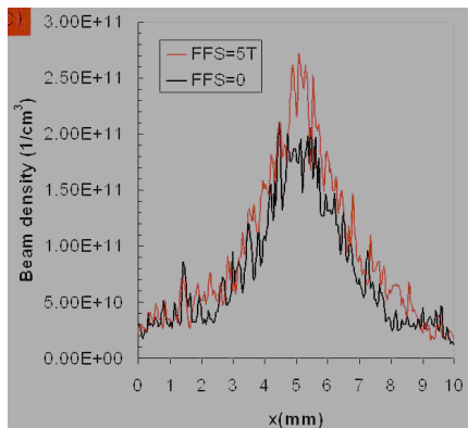
Figure 2: Beam density profiles at the target focal plane with the final focus solenoid on (FFS=5T) and off (FFS=0). The corresponding focal spot FWHM = 2 mm with FFS=5T and 3 mm with FFS=0
