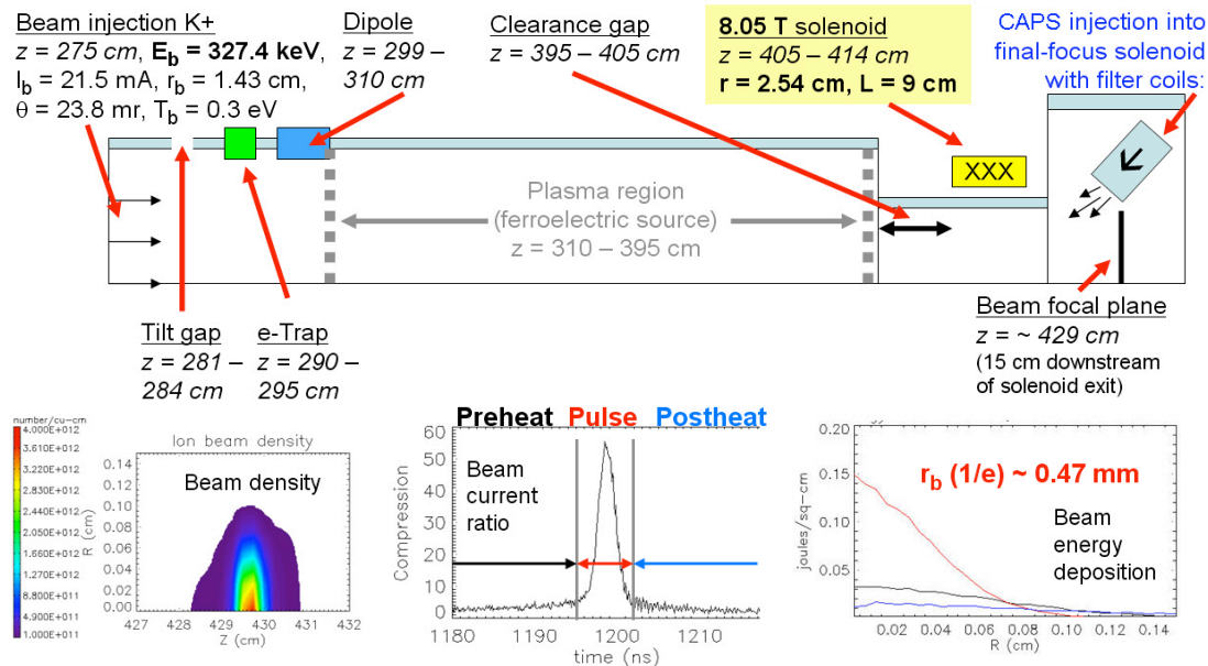
Figure 3: (Top) The simulation model includes the acceleration gap, electrostatic electron trap, permanent magnetic dipole FEPS, clearance gap, final-focus solenoid, and (FCAPS0). The peak beam density (left) reached 4 \times 10^{12} cm -3 , the longitudinal current compression ratio was approximately 55X (middle), and the simultaneous radial spot size (1/e) was 0.47 mm (0.9 mm FWHM) with a peak on-axis cumulative energy deposition of 0.15 J cm -2 (right). The middle and right plots are color coded to show the degree of pre-heat (200 ns total) on the target expected in this configuration.
